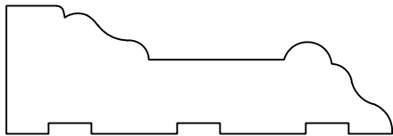
CASG066 3/4" X 2 1/4"
