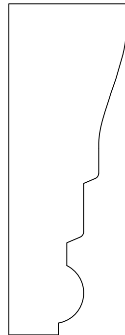
CRWNO12 1 1/4" X 3 1/2"
