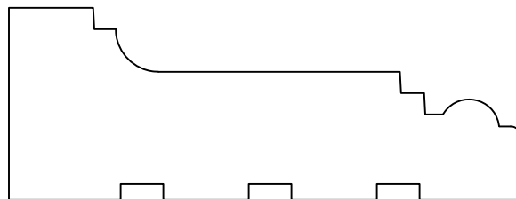
CASG082 1 1/8" X 3"
