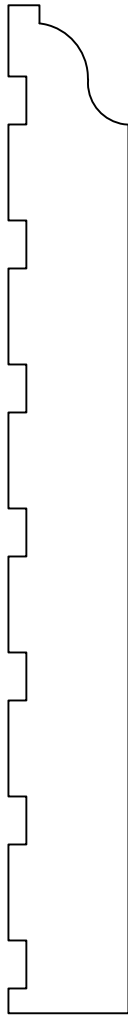
BASE036 5/8" X 5 1/4"
