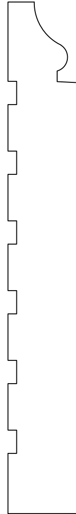
BASE054 3/4" x 5 1/2"
