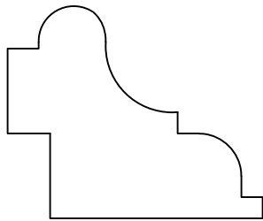
TRIM043 1 1/4" X 1 1/2"
