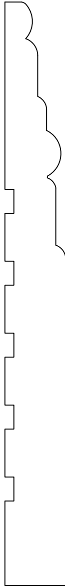
BASE061 5/8" x 6"
