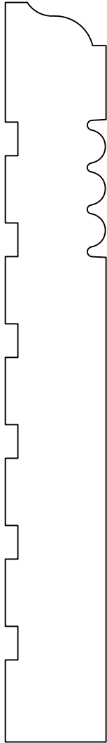
BASE049 3/4" x 5 1/2"
