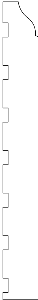
BASE004 5/8" X 5 1/4"
