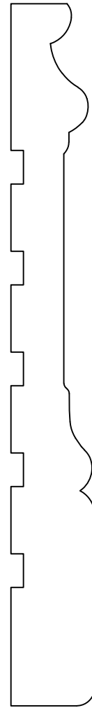
BASE077 5/8" X 5 1/4"
