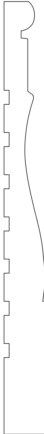
BASE042 3/4" X 7 11/16"
