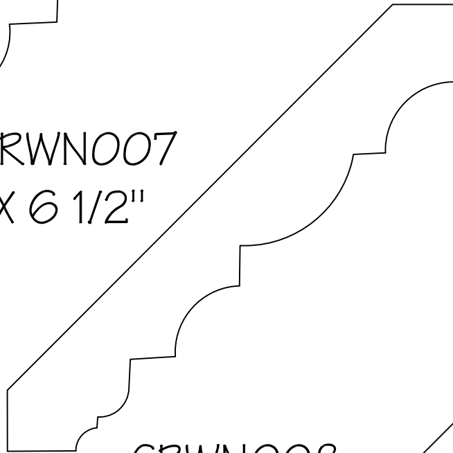
CRWN008 3/4" X 4 3/4"
