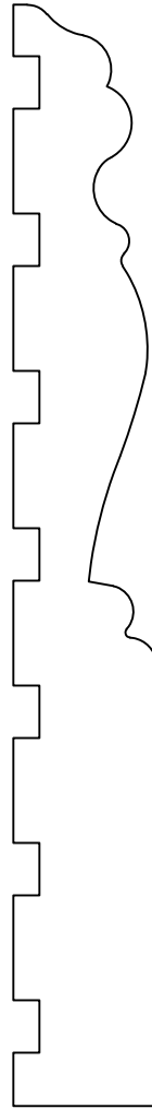
BASE038 11/16" X 5 1/4"
