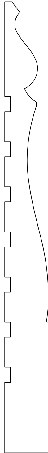
BASE060 3/4" x 7 1/2"
