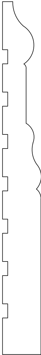
BASE052 11/16" X 6 1/4"
