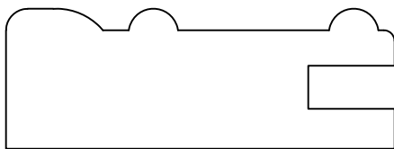
TRIM032 13/16" X 2 1/4"
