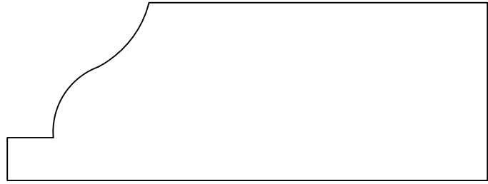
TRIM108 1 5/16" x 3 1/2"
