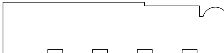
CASG104 7/8" x 3 3/4"
