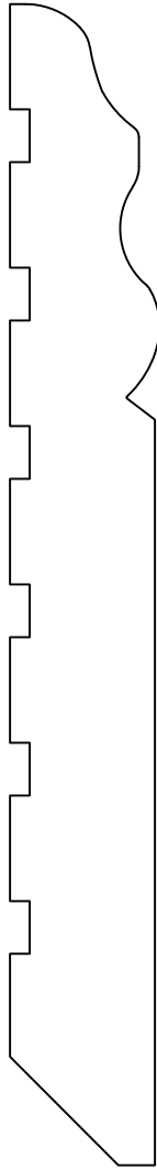
BASE055 11/16" x 5 1/2"
