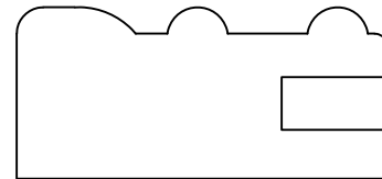
TRIM033 13/16" X 1 3/4"
