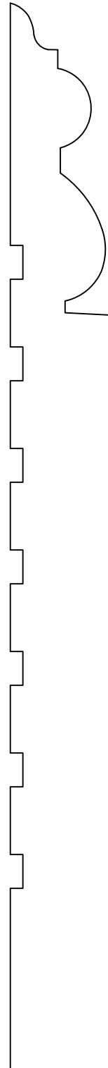
BASE051 3/4" x 7 7/8"
