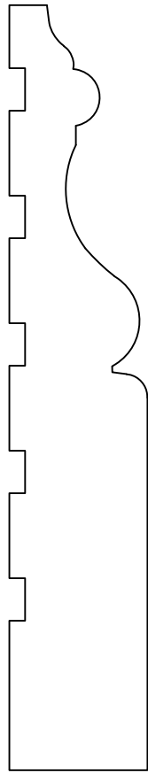
BASE011 13/16" X 4 1/2"
