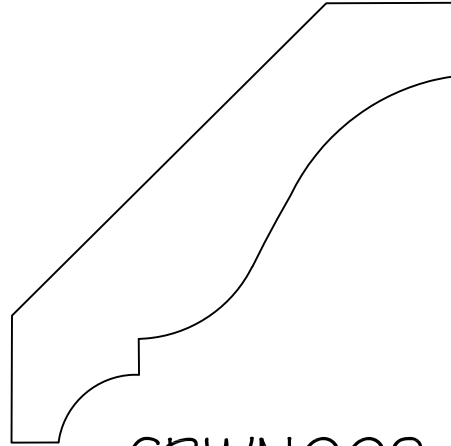
CRWN002 3/4" X 3 1/4"
