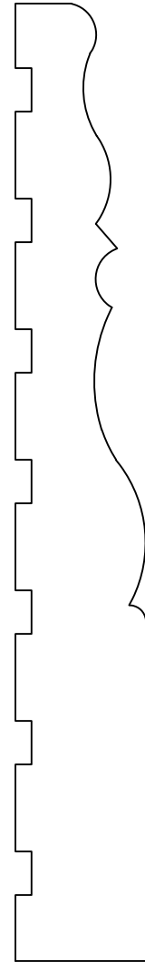
BASE031 3/4" X 5 1/2"
