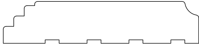
CASG105 3/4" x 3 1/2"
