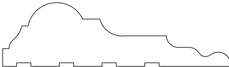
CASG015 1 1/8" X 4"
