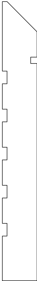
BASE083 11/16" X 5 1/2 "
