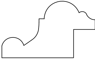
TRIM061 1" x 1 5/8"
