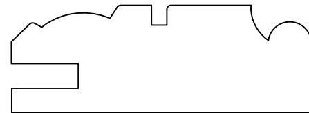
TRIM064 13/16" x 2 1/4"
