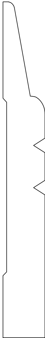
BASE076 3/4" X 6"
