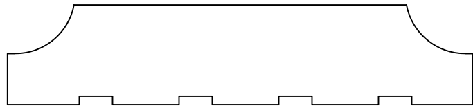
CASG021 3/4" X 3 1/2"
