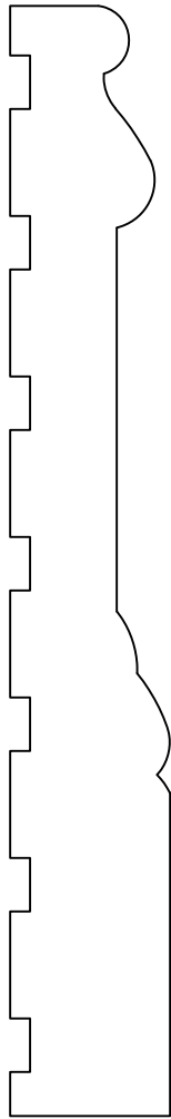
BASE020 3/4" X 5 3/16"
